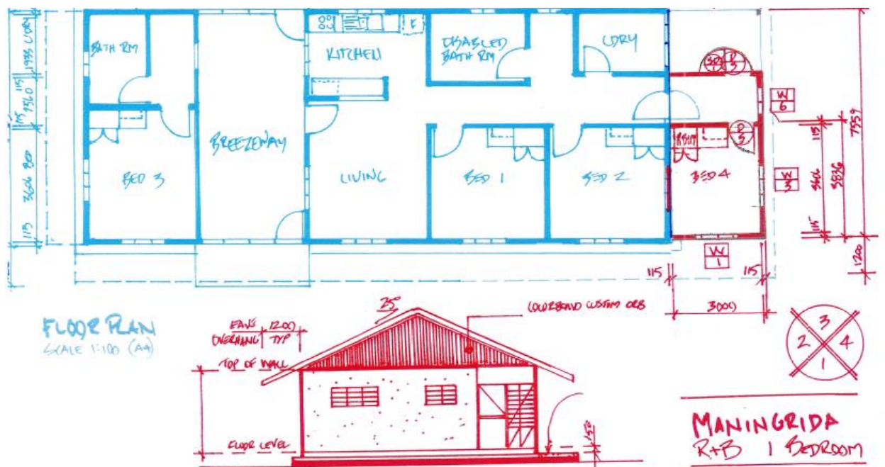
Concept plan only: Maningrida - modify 7 dwellings
