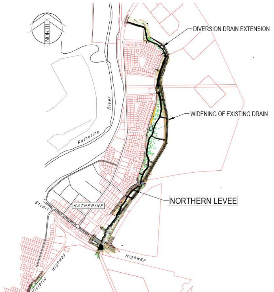
Location plan: Flood Mitigation - levee construction
