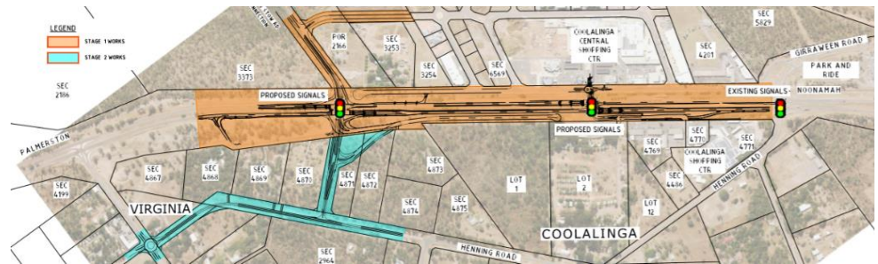
Concept: Coolalinga commercial precinct access - improve safety and connectivity
