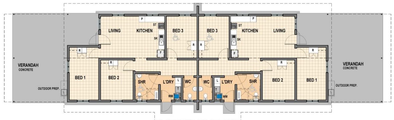
Concept (standard design): Maningrida - HomeBuild NT - construct 3 bedroom duplex
