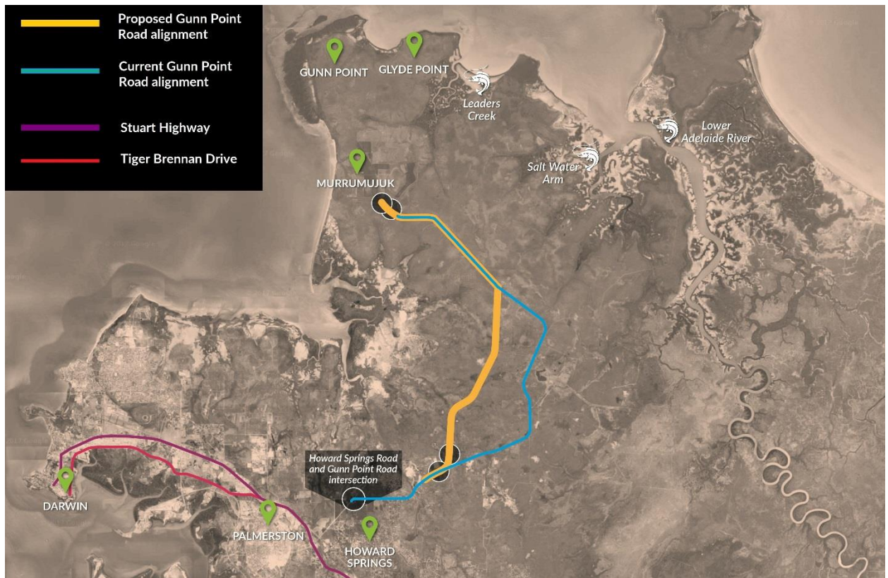
Map: Gunn Point Road - alignment
