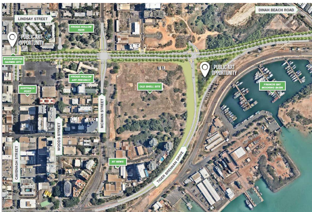
Location map: Darwin CBD - Barneson Boulevard Link - duplication of Tiger Brennan Drive from Dinah Beach to McMinn Street (stage 3)
