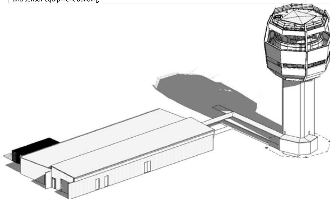
Concept: RAAF Base Tindal - Air 5431 - air traffic control - construct new 25m high multi-level facility and sensor equipment building
