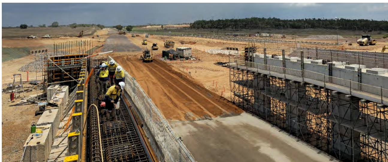
Tiger Brennan Drive - design and construct overpass at Berrimah Road intersection
